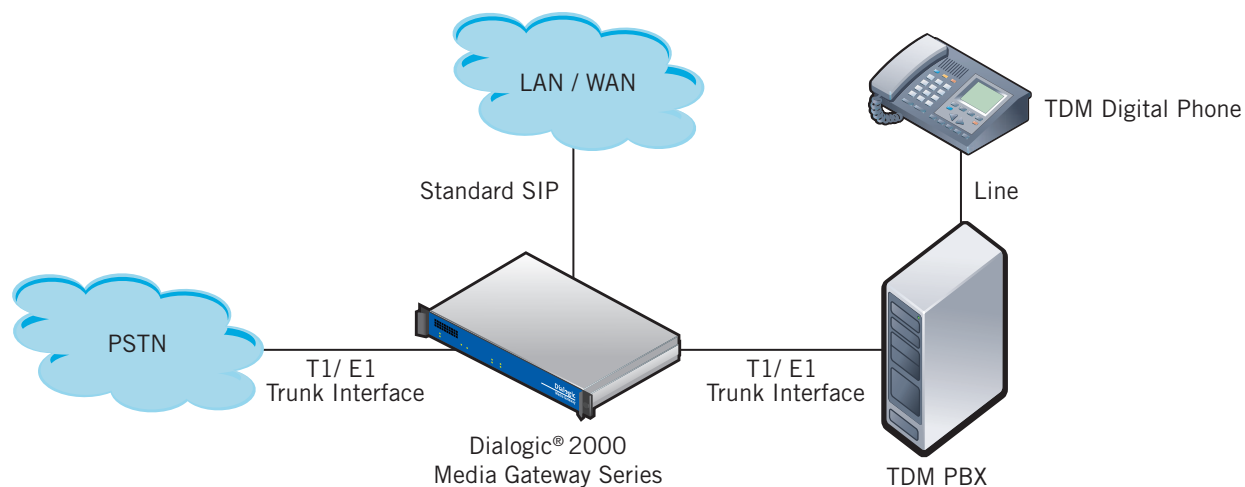
Figure 4. Access Gateway with Survivability Capabilities
