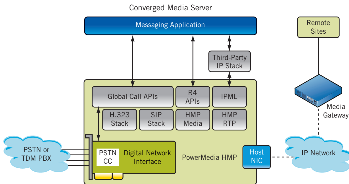
Figure 3. Converged Media Server Architecture
